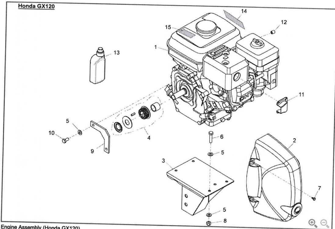
Engine Assembly (Honda GX120)
