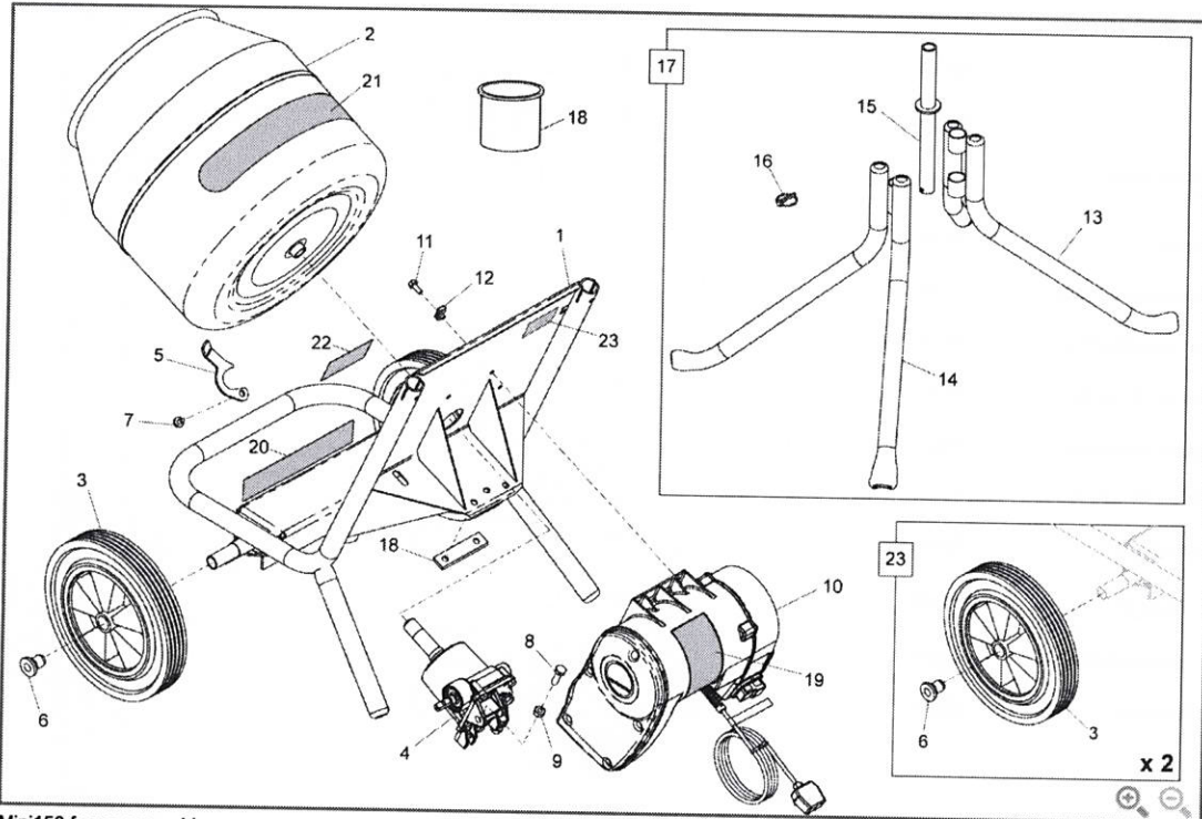
Mini150 frame assembly
